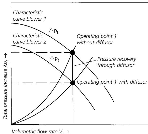
Figure 2: Pressure recovery
