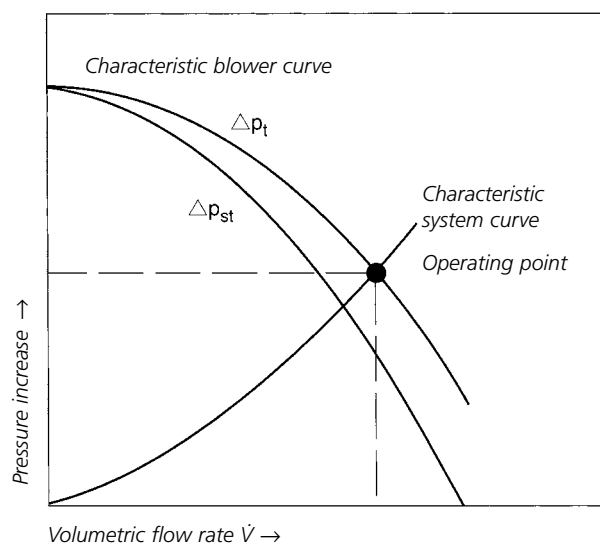
Figure 1: Operating point of the blower
